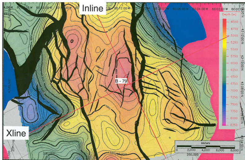
Figure 121. Top structure map for the C32 target zone at Balvenie B-79 (Balvenie ADW, used with permission).
